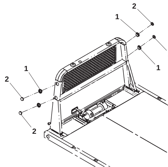
FOR 45", 50" & 57" HEADBOARD
